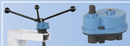
No. 6587 – 2:1 reduction gearbox. Allows a 2:1 torque compression increase when compressing struts.
